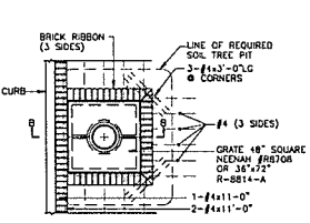
STREET TREE PLANTING DETAIL SCALE 3/8"=1'-0"
