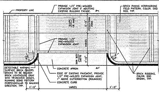
CURB CUT DETAIL SCALE 1/16"=1'-0"
