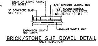
BRICK/STONE SLIP DOWEL DETAIL SCALE 3/4"=1'-0"
