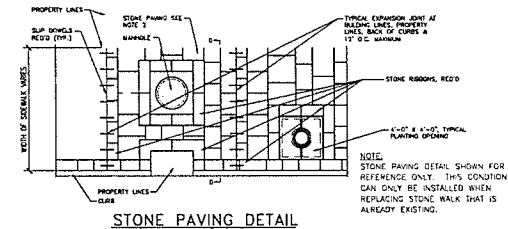
STONE PAVING DETAIL SCALE 1/4"=1'-0"
