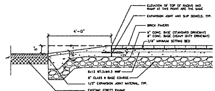
SECTION A-A SCALE 3/4"=1'-0"
