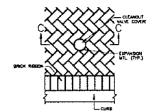
CLEANOUT OR VALVE TYPICAL PLAN SCALE 3/4"=1'-0"
