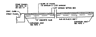
SECTION D-D SCALE 1/4"=1'-0"
