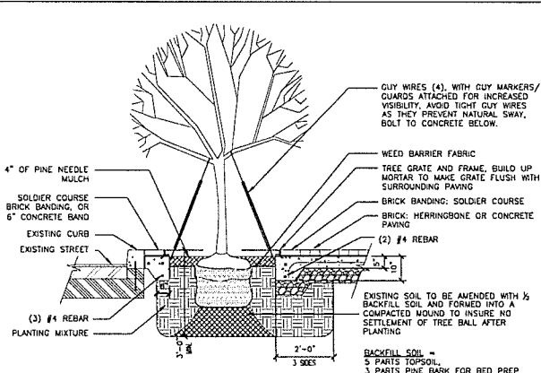
SECTION B-B SCALE 3/4"=1'-0"
