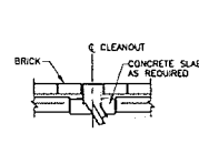
SECTION C-C SCALE 3/4"=1'-0"
