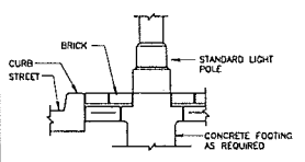
TYPICAL POLE SECTION SCALE 3/4"=1'-0"
