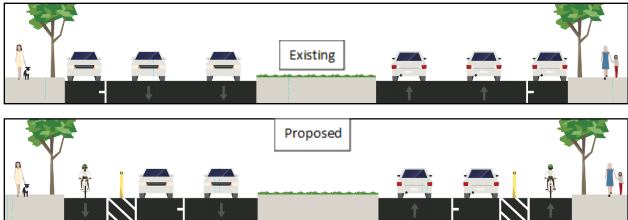
Existing and proposed typical roadway cross sections for Paris Avenue (I-610 and Filmore Avenue)
